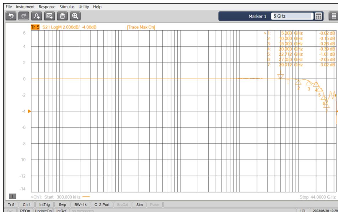
Insertion loss
