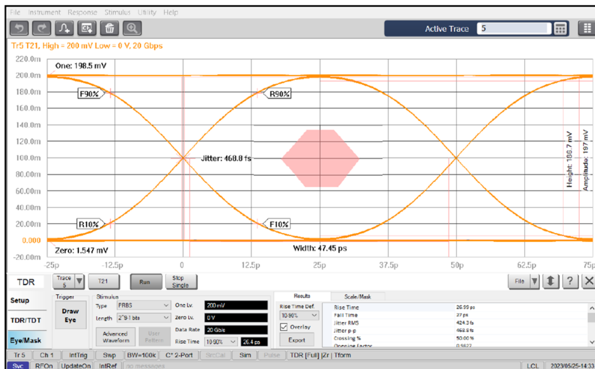
Eye pattern
