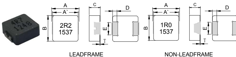
LEADFRAME
