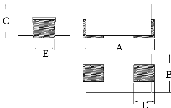
Dimensions: C8B 403025
