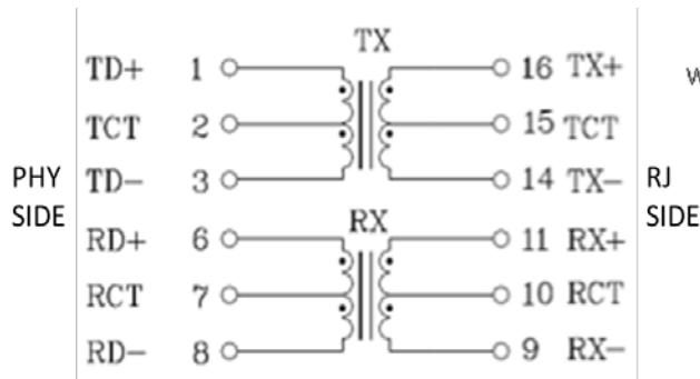
LAN-12M162P7B0
