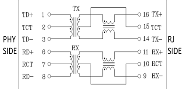
LAN-12M162P7B0
