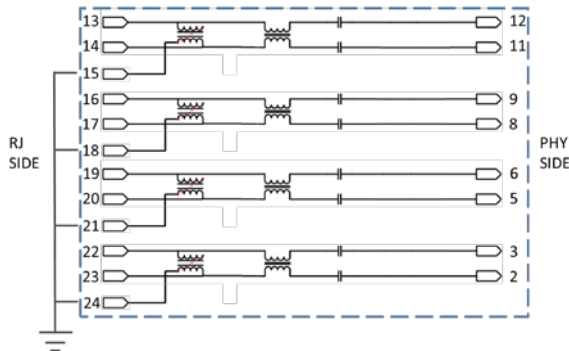
LAN-16G241S1A8
