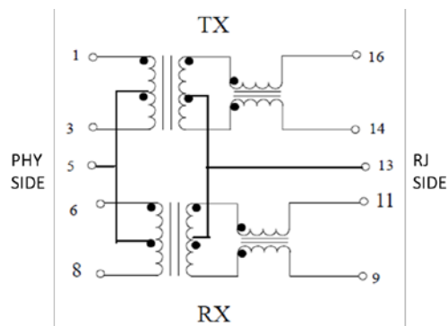
LAN-12M165P7A8
