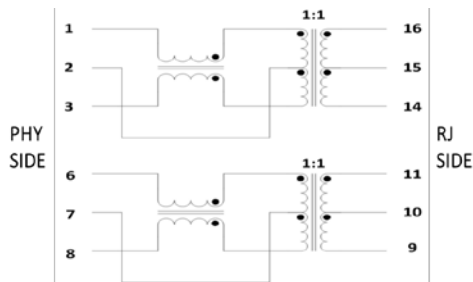
LAN-12M165P7A8
