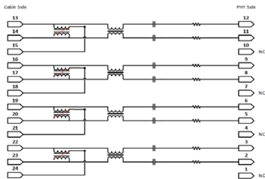
LAN-16G241S1B8
