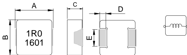
non-leadframe
